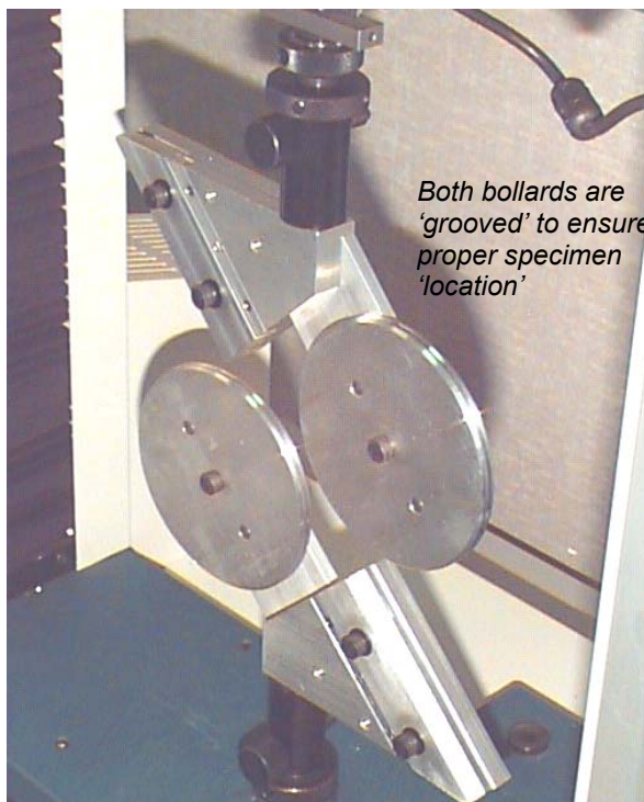
View of Grip attachments assembled on model H10KS and ready for test
