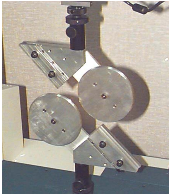
View of Grip attachments assembled on model H10KS and ready for test
