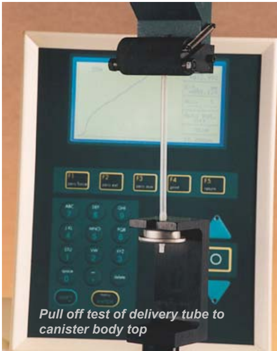
Separation test (Tensile) of packaging
