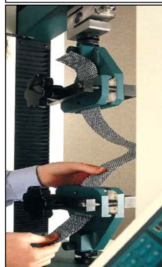
Stretch Recovery Tests
