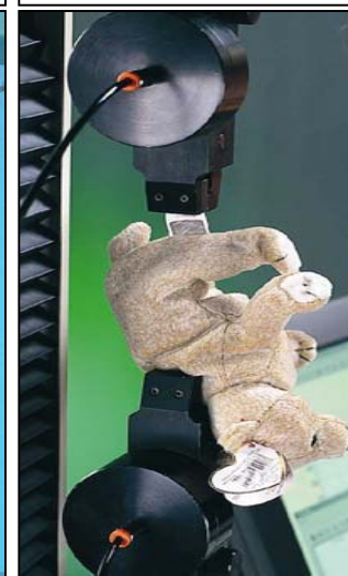
Toy Tests using pneumatic grips
