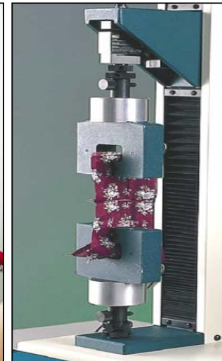
Seam slippage tests using pneumatic grips
